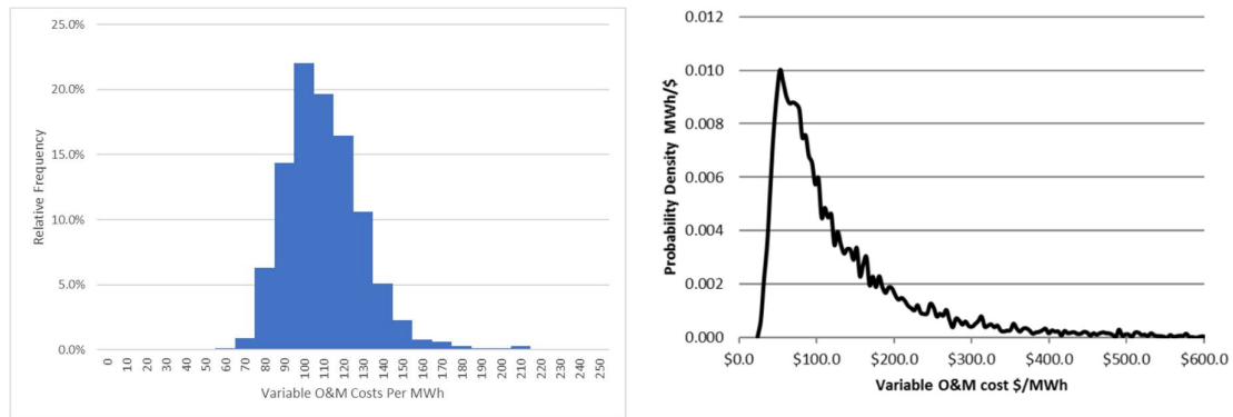
Figure 19: Comparison of PDF for Variable O&M Costs ($ per MWh) – Pinjar Units 2019-20 (left) and 2018-19 (right)
