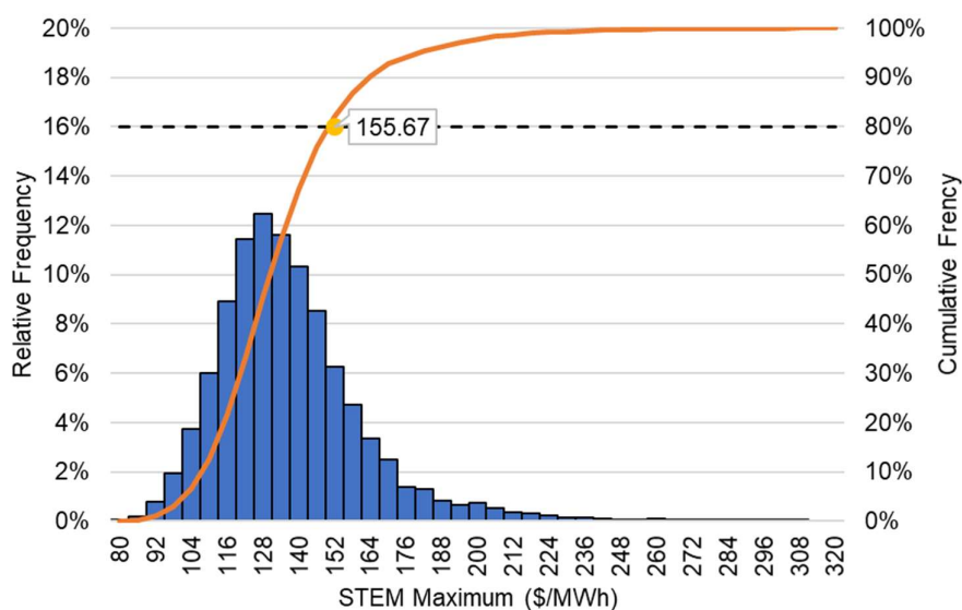
Figure 14: Maximum STEM Price probability density function – Parkeston Units
