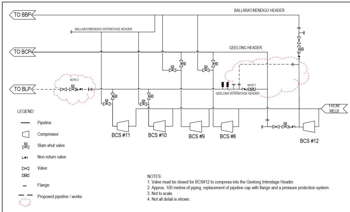
Figure 11 Proposed reconfiguration of Brooklyn Compressor Station
