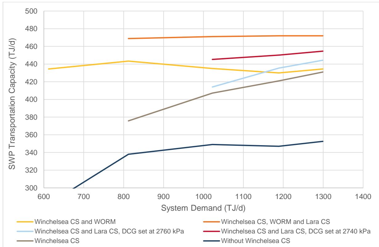
Figure 15 South West Pipeline capacity to Melbourne with Western Outer Ring Main and Lara Compressor Station
