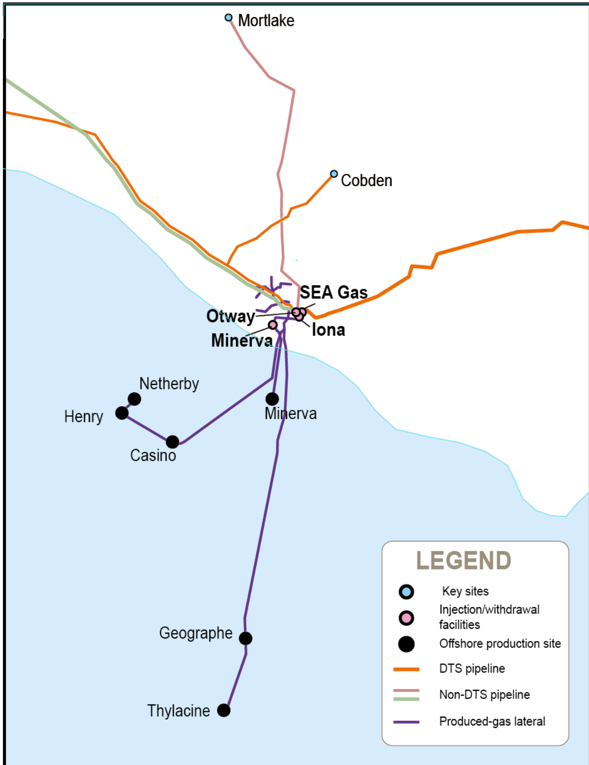
Figure 5 Map of Port Campbell gas production facilities
