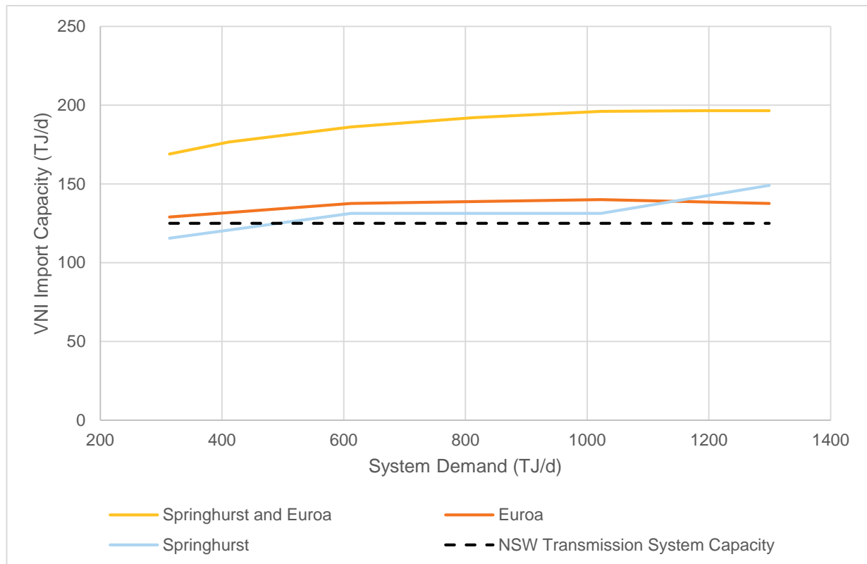
Figure 4 Victorian Northern Interconnect import capacity post winter 2016 expansion
