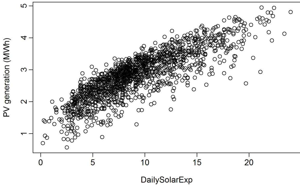
Figure 39: Daily solar PV generation plotted against daily solar exposure data in VIC from 2003 to 2011. Only data from April–September are shown.
