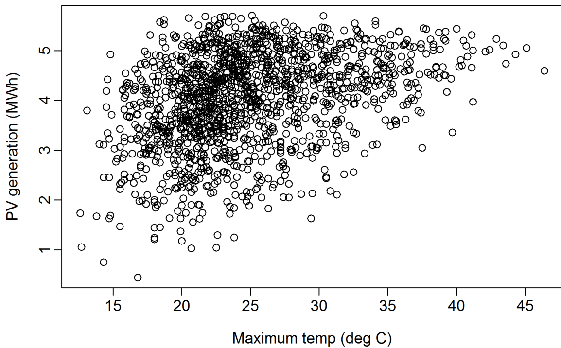
Figure 15: Daily solar PV generation plotted against daily maximum temperature in VIC from 2003 to 2011. Only data from October–March are shown.
