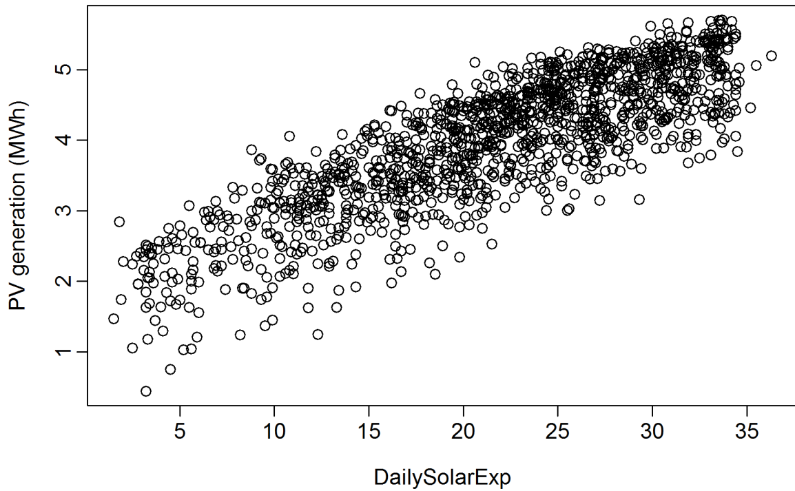
Figure 14: Daily solar PV generation plotted against daily solar exposure data in VIC from 2003 to 2011. Only data from October–March are shown.
