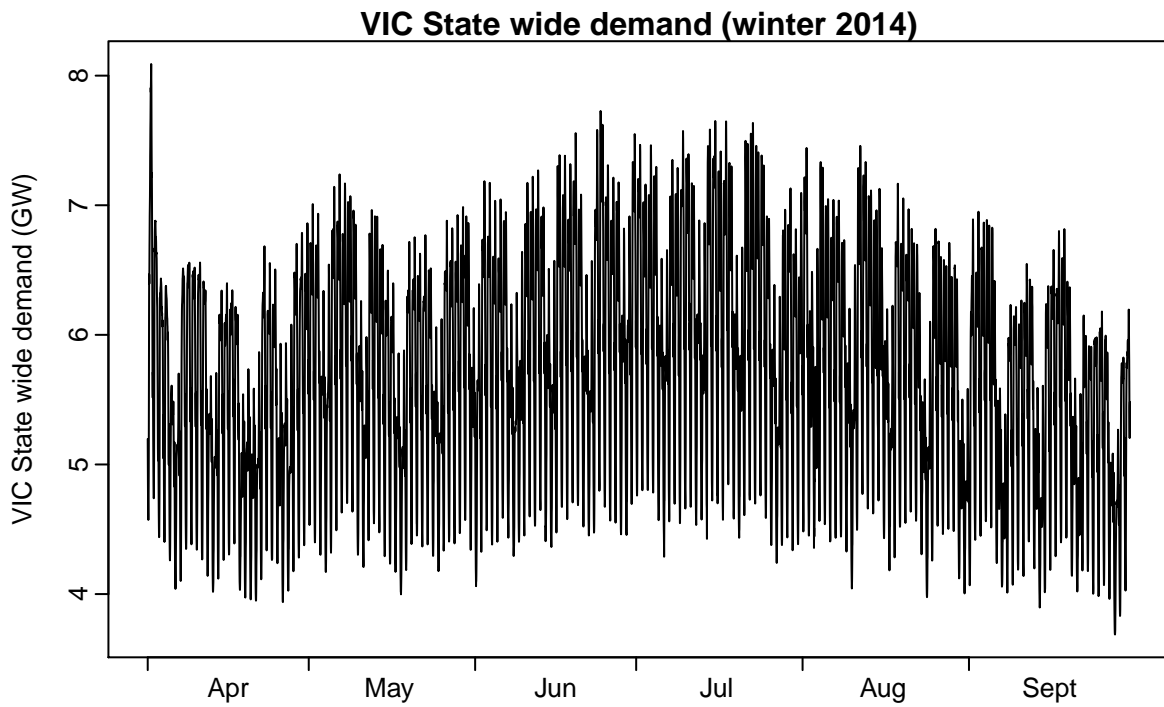
Figure 28: Half-hourly demand data for Victoria for last winter.
