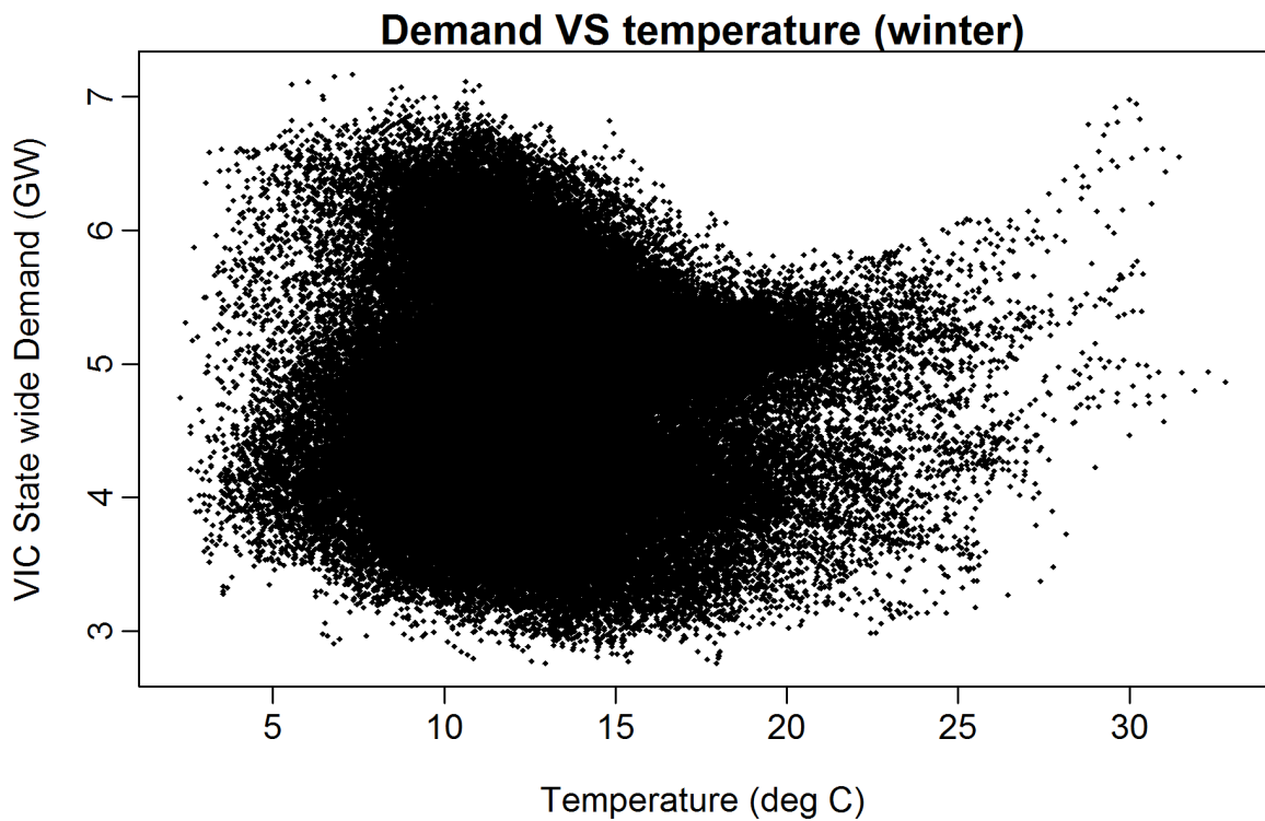
Figure 33: Half-hourly VIC electricity demand (excluding major industrial demand) plotted against average temperature (degrees Celsius).
