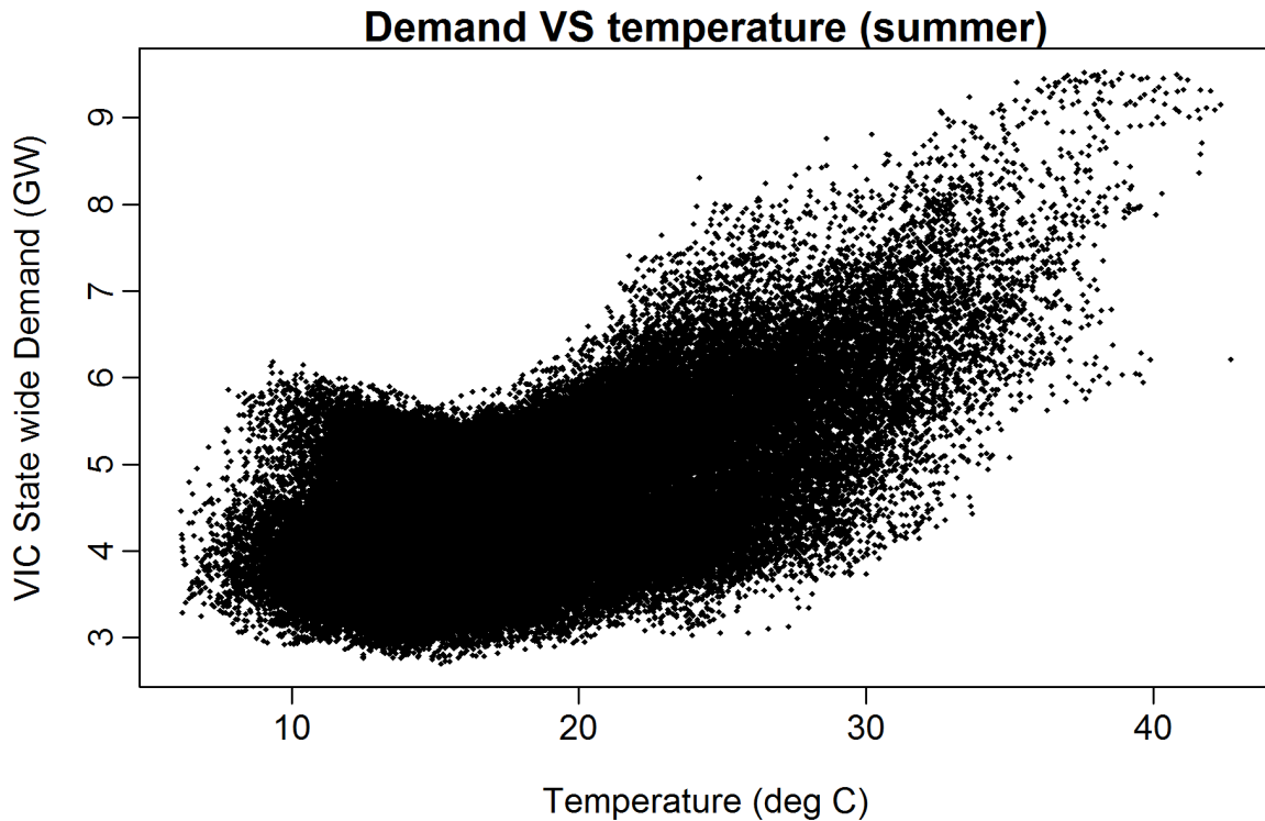
Figure 7: Half-hourly VIC electricity demand (excluding major industrial demand) plotted against average temperature (degrees Celsius).
