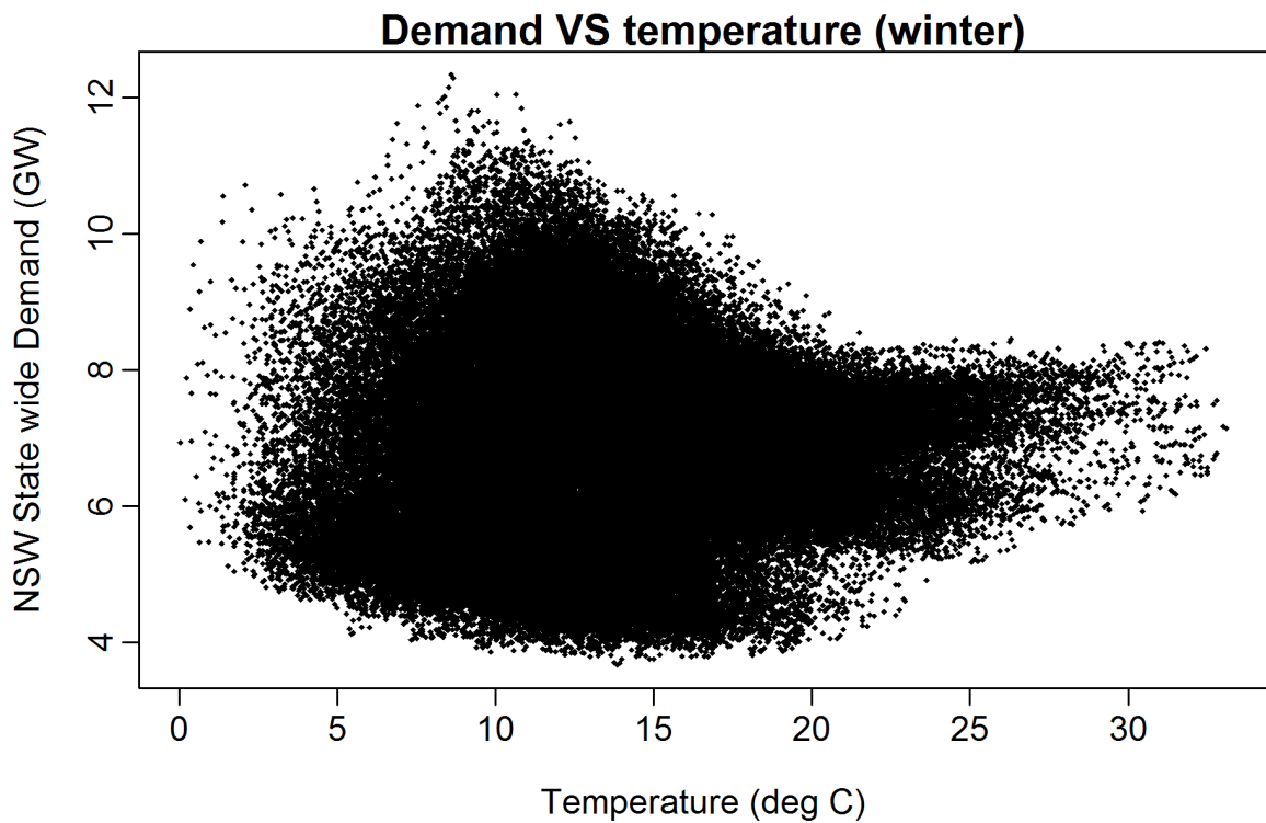
Figure 33: Half-hourly NSW electricity demand (excluding major industrial demand) plotted against average temperature (degrees Celsius).
