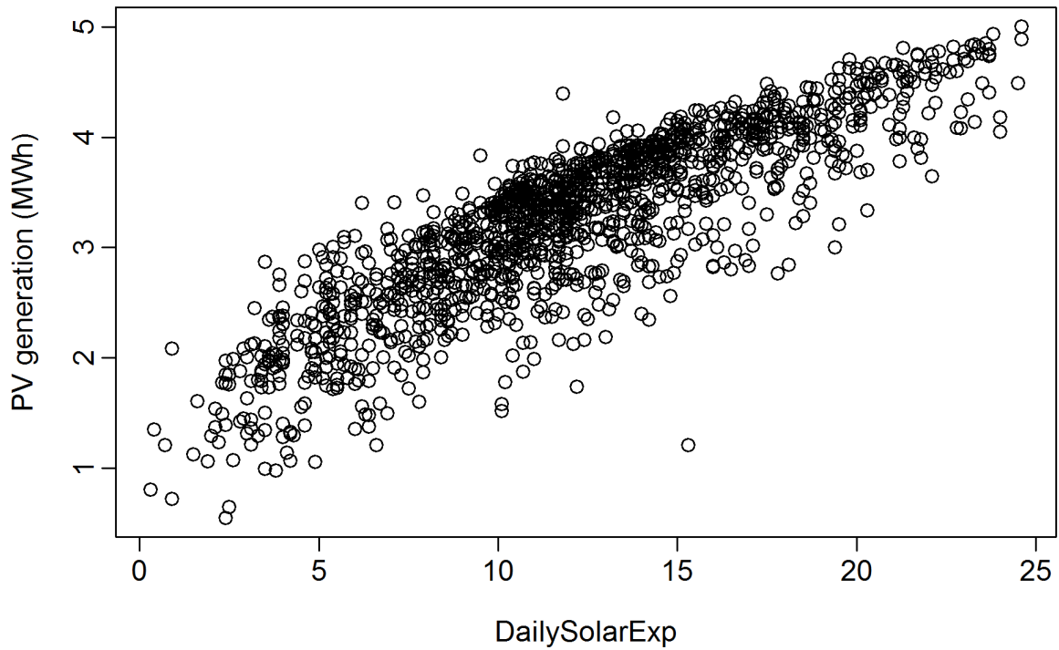
Figure 39: Daily solar PV generation plotted against daily solar exposure data in NSW from 2003 to 2011. Only data from April–September are shown.
