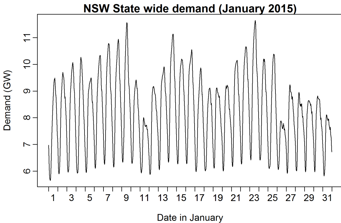
Figure 3: Half-hourly demand data for New South Wales, January 2015.
