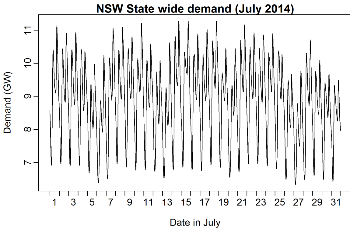
Figure 29: Half-hourly demand data for New South Wales, July 2014.
