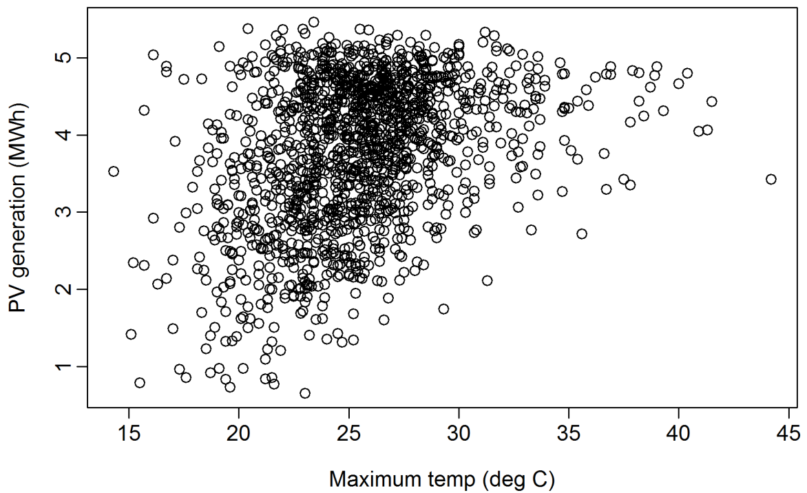
Figure 15: Daily solar PV generation plotted against daily maximum temperature in NSW from 2003 to 2011. Only data from October–March are shown.
