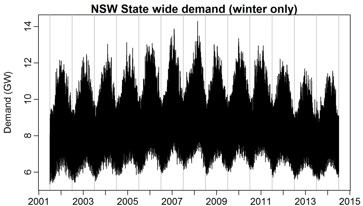
Figure 27: Half-hourly demand data for New South Wales from 2002 to 2015. Only data from April–September are shown.
