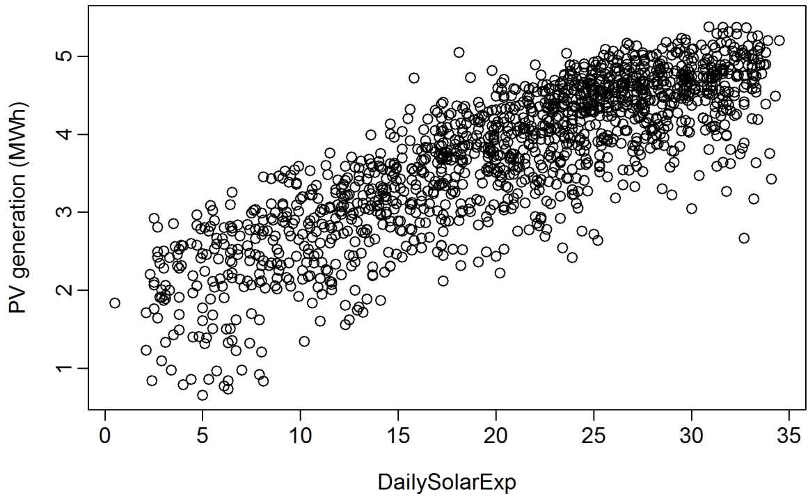
Figure 14: Daily solar PV generation plotted against daily solar exposure data in NSW from 2003 to 2011. Only data from October–March are shown.
