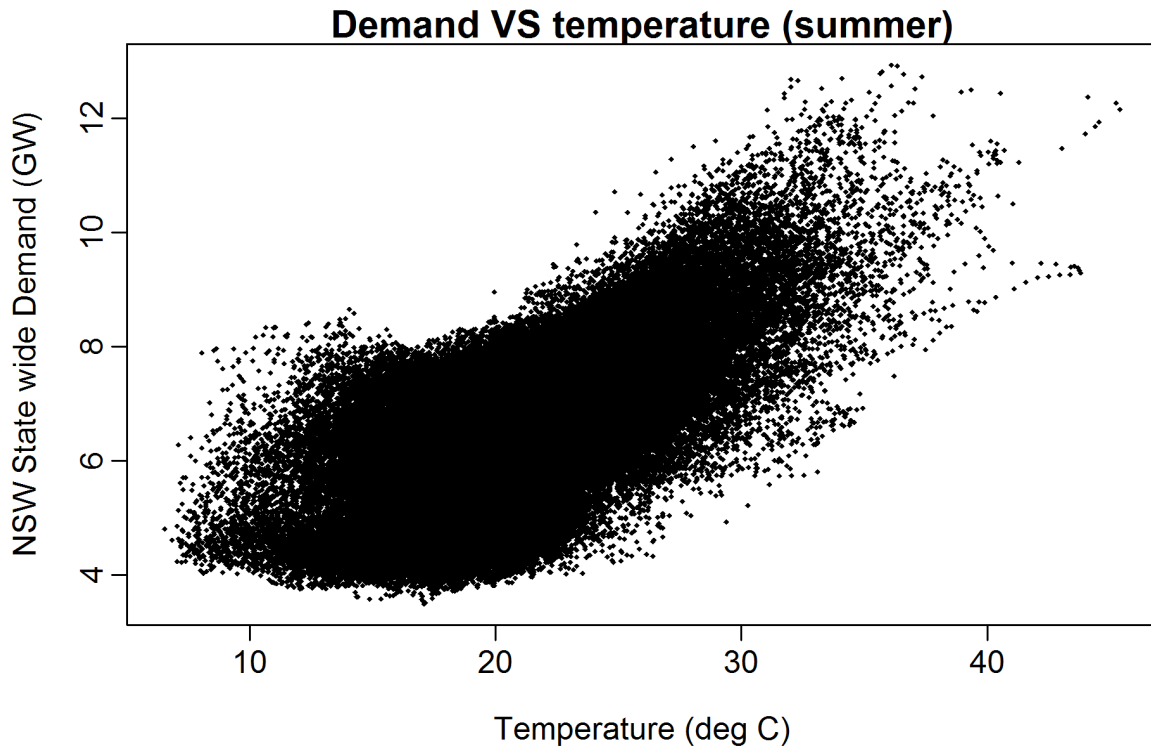
Figure 7: Half-hourly NSW electricity demand (excluding major industrial demand) plotted against average temperature (degrees Celsius).
