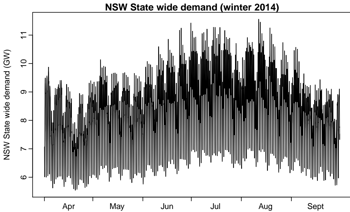
Figure 28: Half-hourly demand data for New South Wales for last winter.
