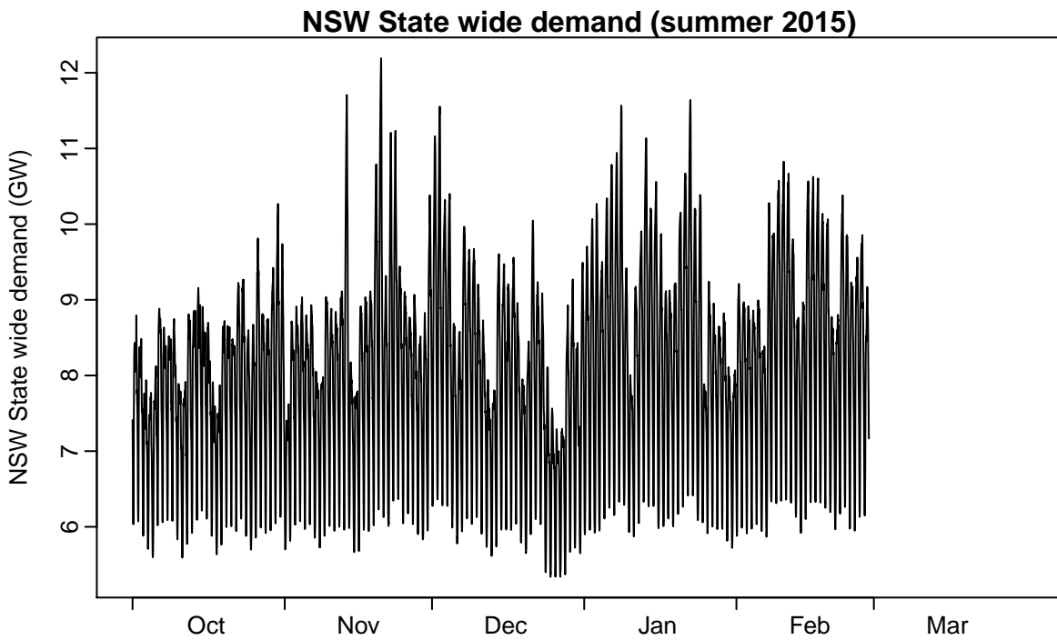
Figure 2: Half-hourly demand data for New South Wales for last summer.
