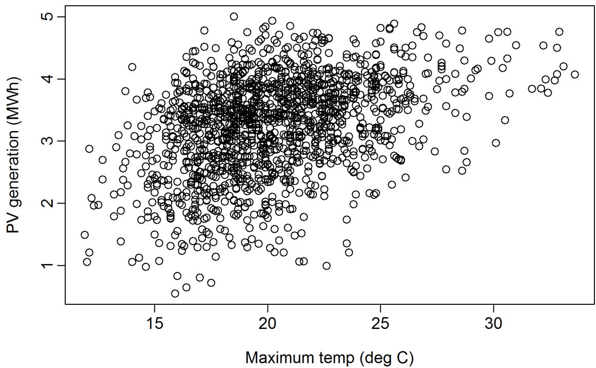
Figure 40: Daily solar PV generation plotted against daily maximum temperature in NSW from 2003 to 2011. Only data from April–September are shown.
