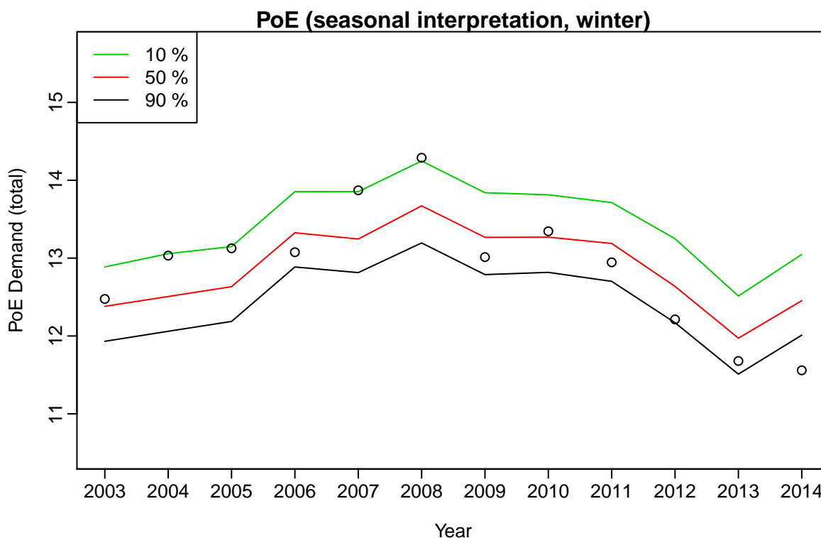
Figure 43: PoE levels of demand excluding offset loads for all years of historical data using known economic values but simulating temperatures.
