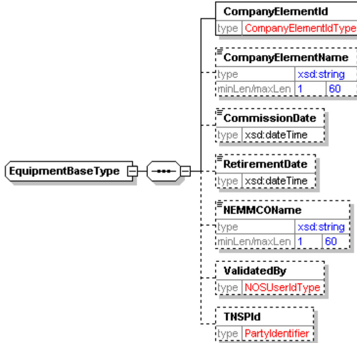
Figure 4-2 EquipmentBaseType Definition
