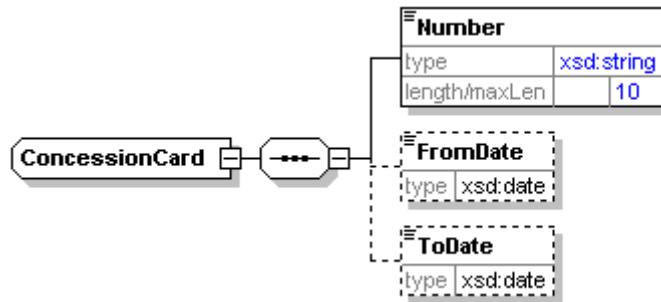
Figure 4-1 ConcessionCard Type Definition
