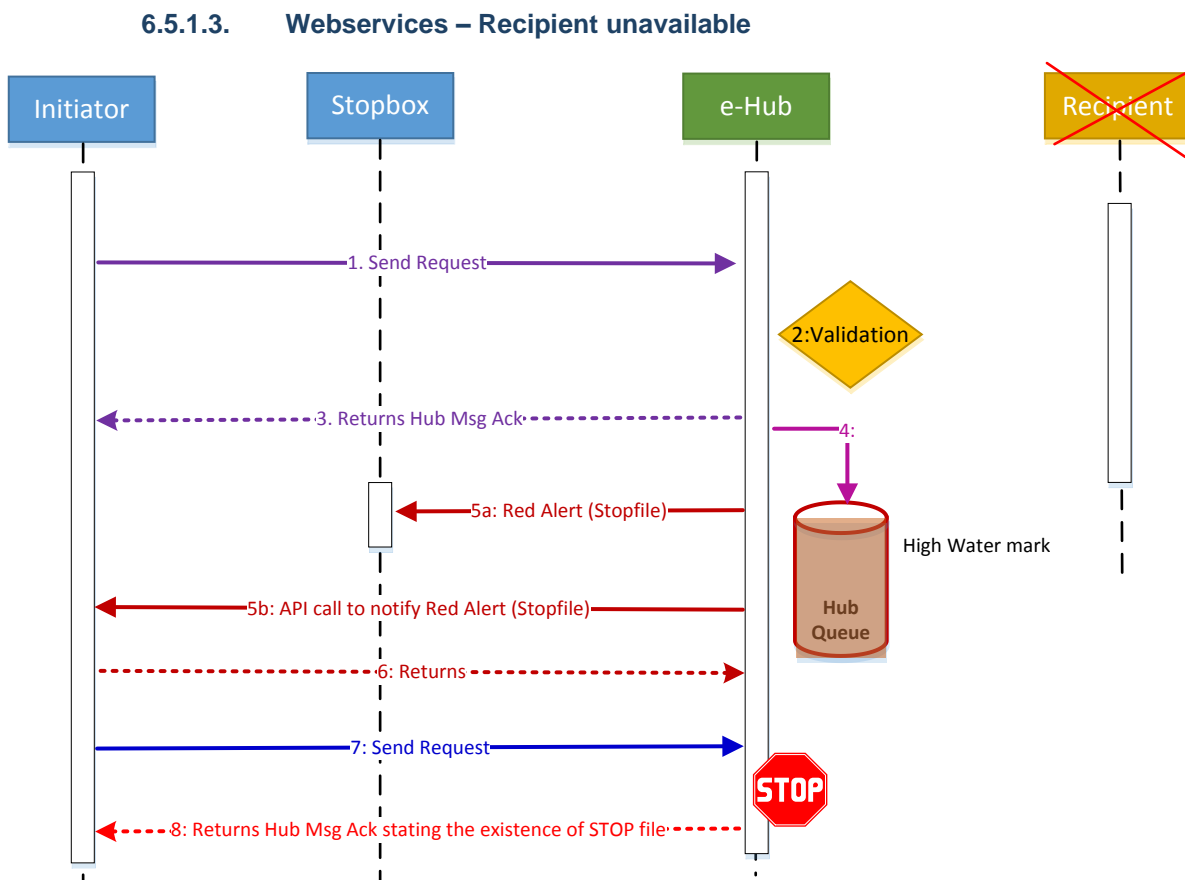
Figure 13: Webservices Sequence Diagram – Acknowledgement Model when Recipient unavailable
