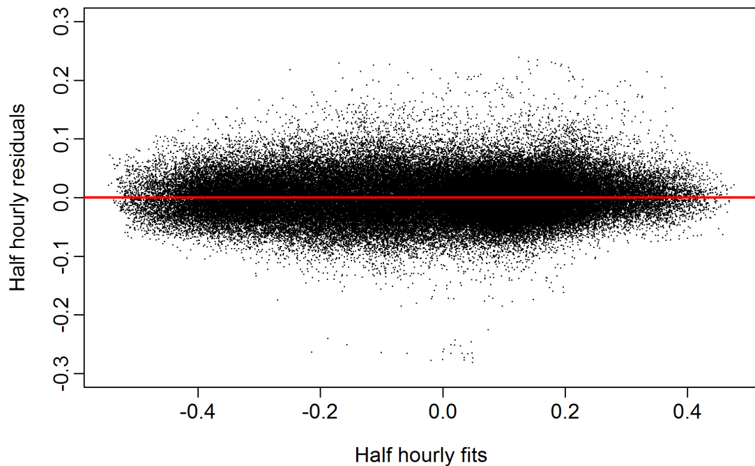
Figure 37: Residuals vs predicted log adjusted demand from the demand model.
