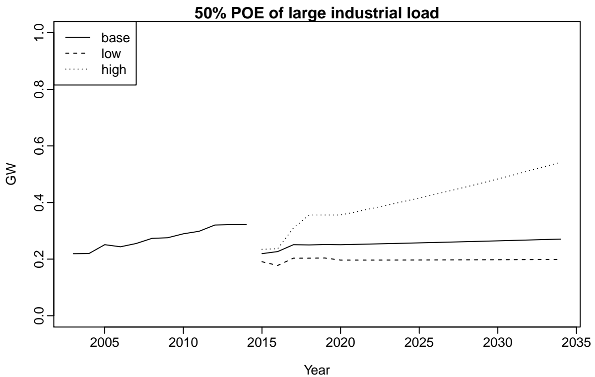
Figure 45: Three scenarios for major industrial loads.
