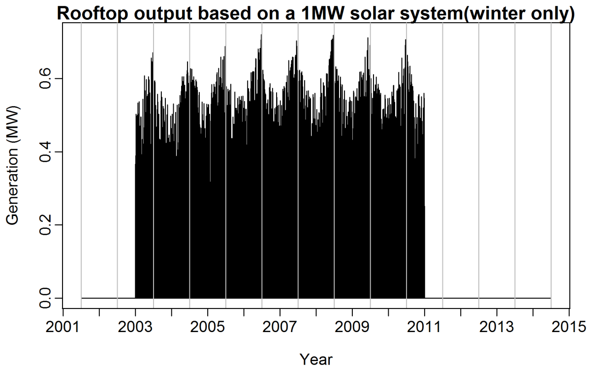
Figure 30: Half-hourly rooftop generation data based on a 1MW solar system. 2003–2011.
