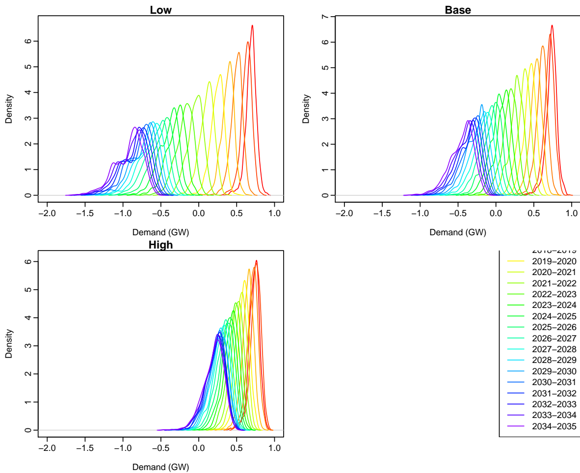
Figure 23: Distribution of simulated seasonal minimum demand for 2015/16–2034/35.
