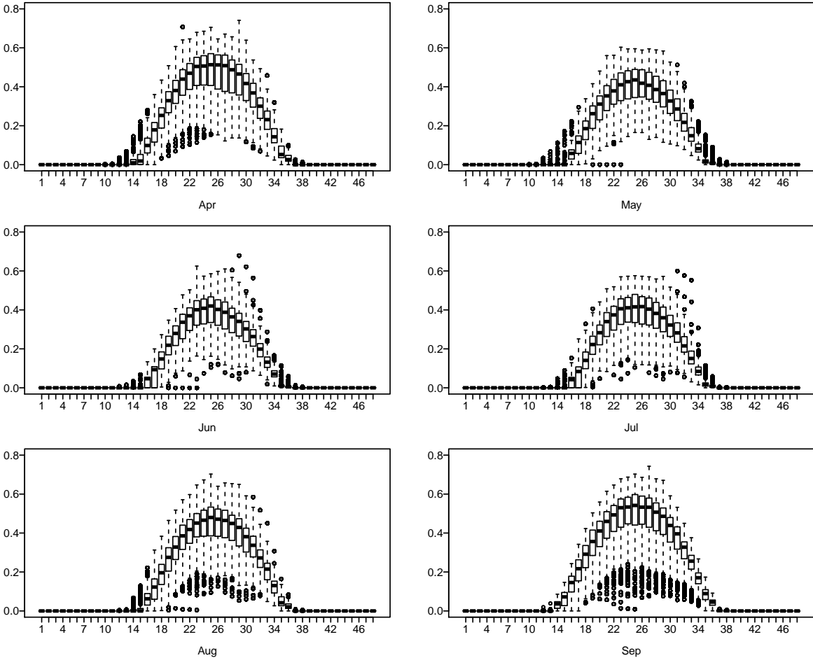
Figure 41: Boxplot of simulated PV output based on a 1 MW solar system. Only data from April–September are shown.
