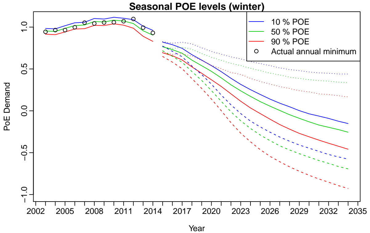
Figure 49: Probability of exceedance values for past and future years. Forecasts based on the base scenario are shown as solid lines; forecasts based on the low scenario are shown as dashed lines; Forecasts based on the high scenario are shown as dotted lines.
