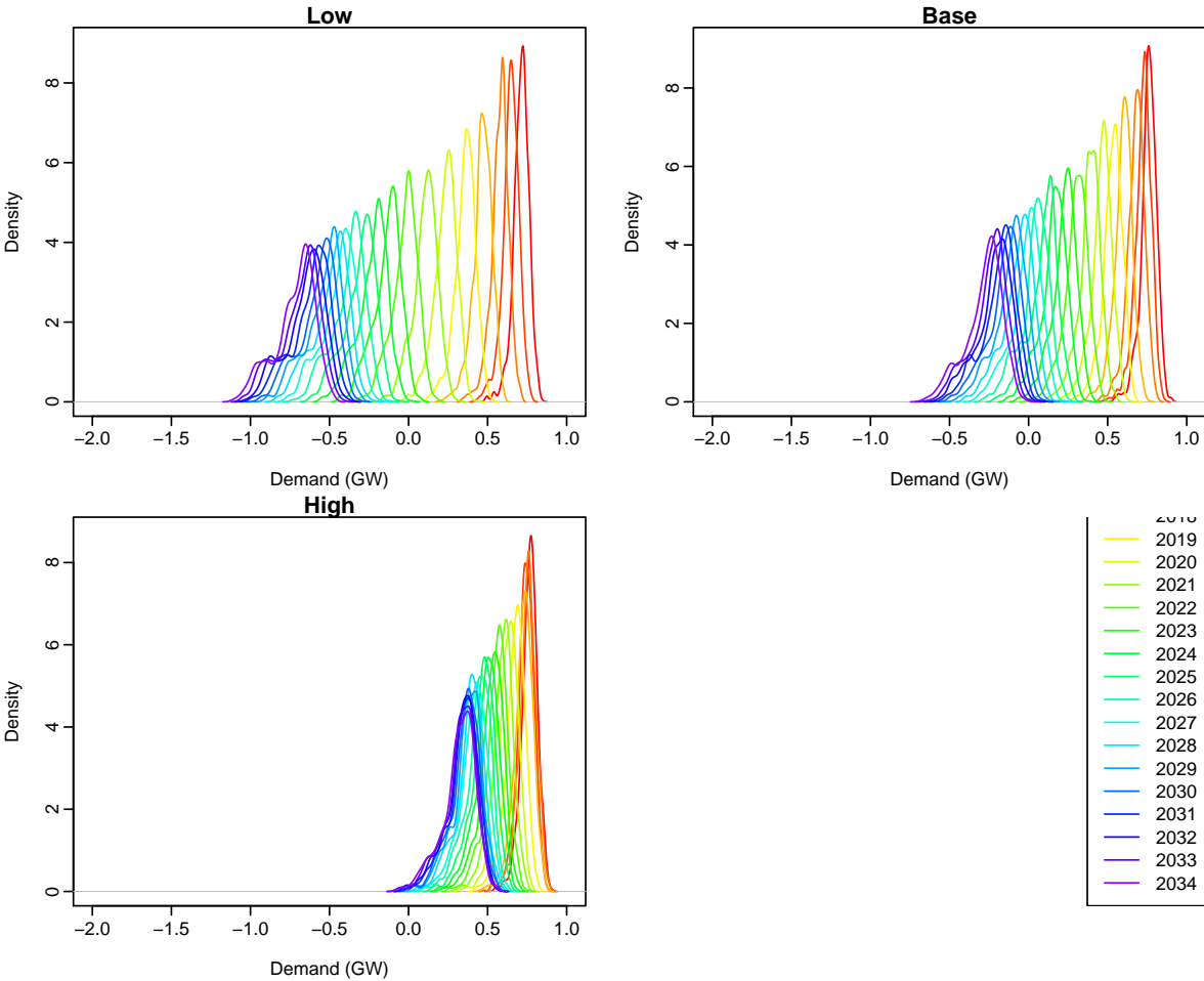
Figure 47: Distribution of simulated seasonal minimum demand for 2015 – 2034.
