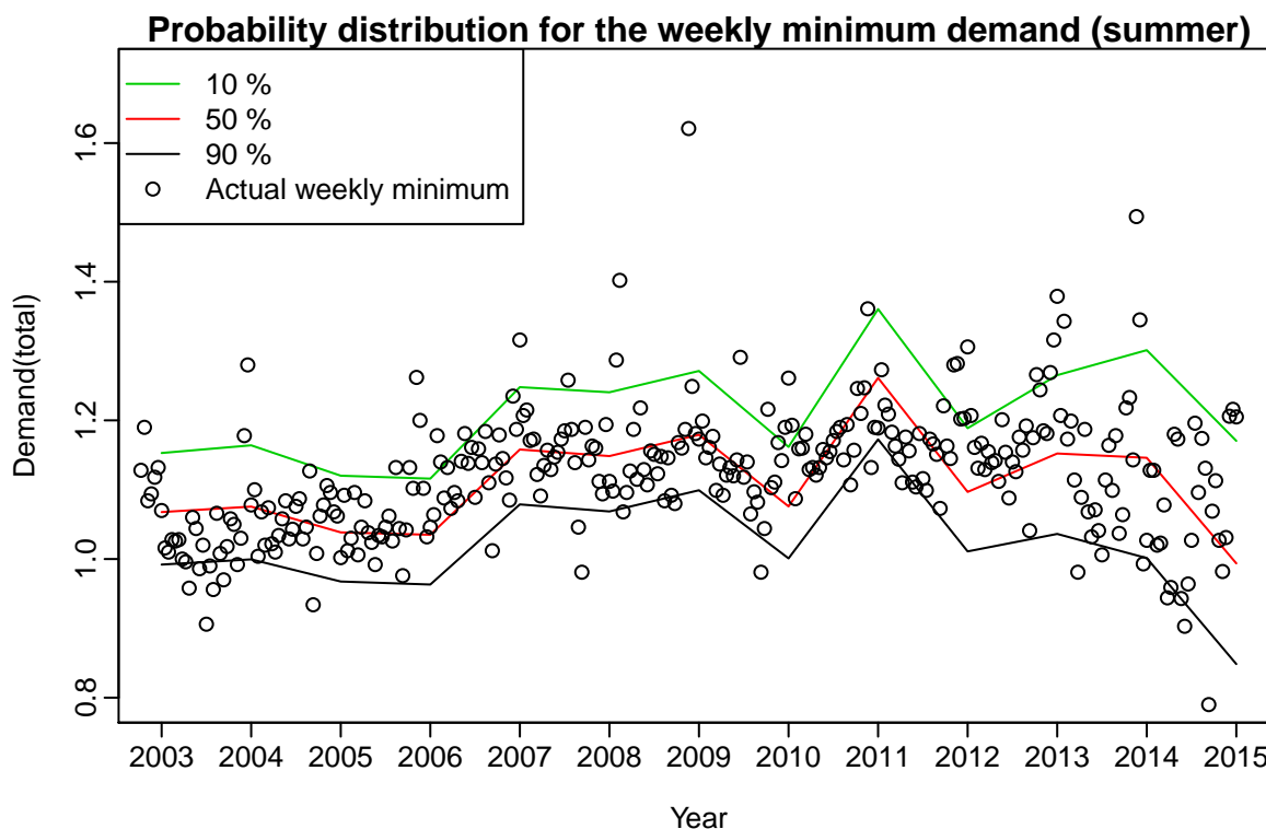
Figure 19: Probability distribution of the weekly minimum demand for all years of historical data using known economic values but simulating temperatures.
