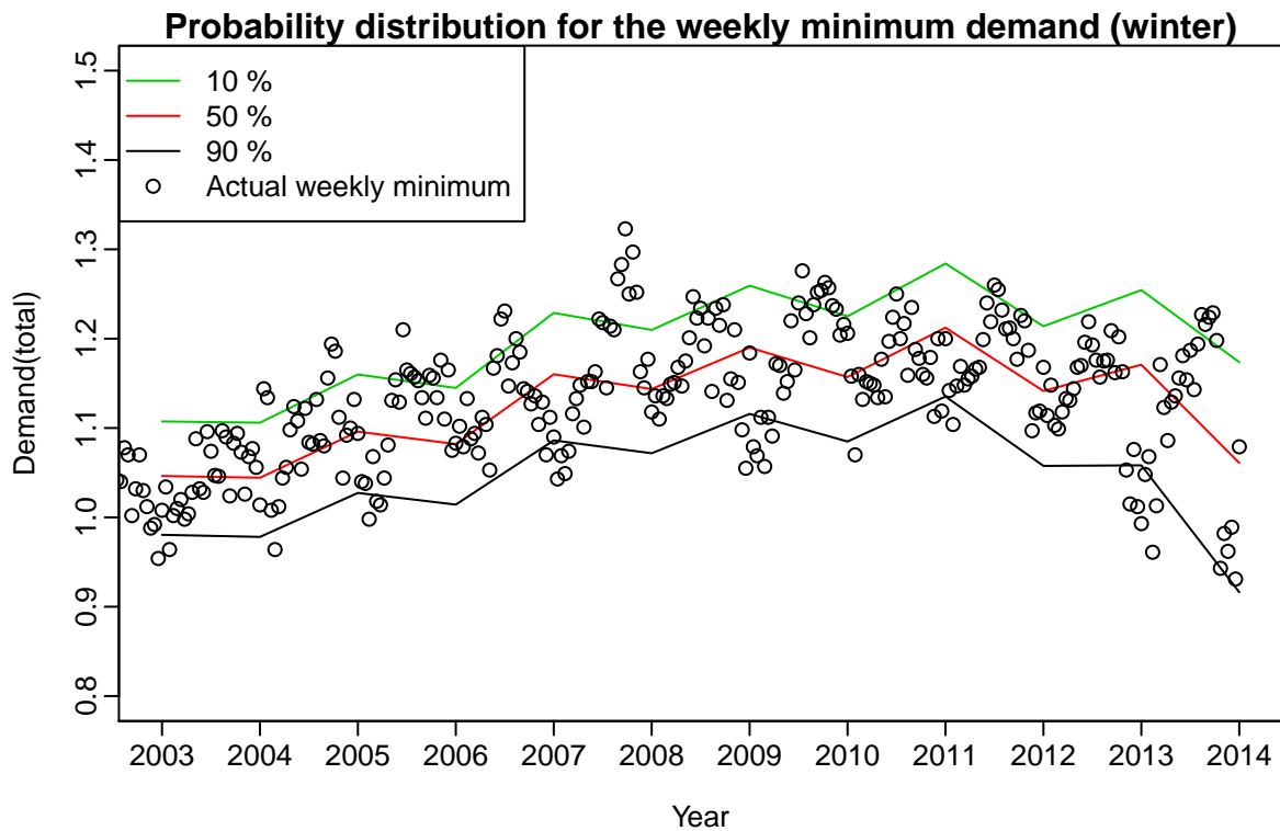
Figure 43: Probability distribution of the weekly minimum demand for all years of historical data using known economic values but simulating temperatures.
