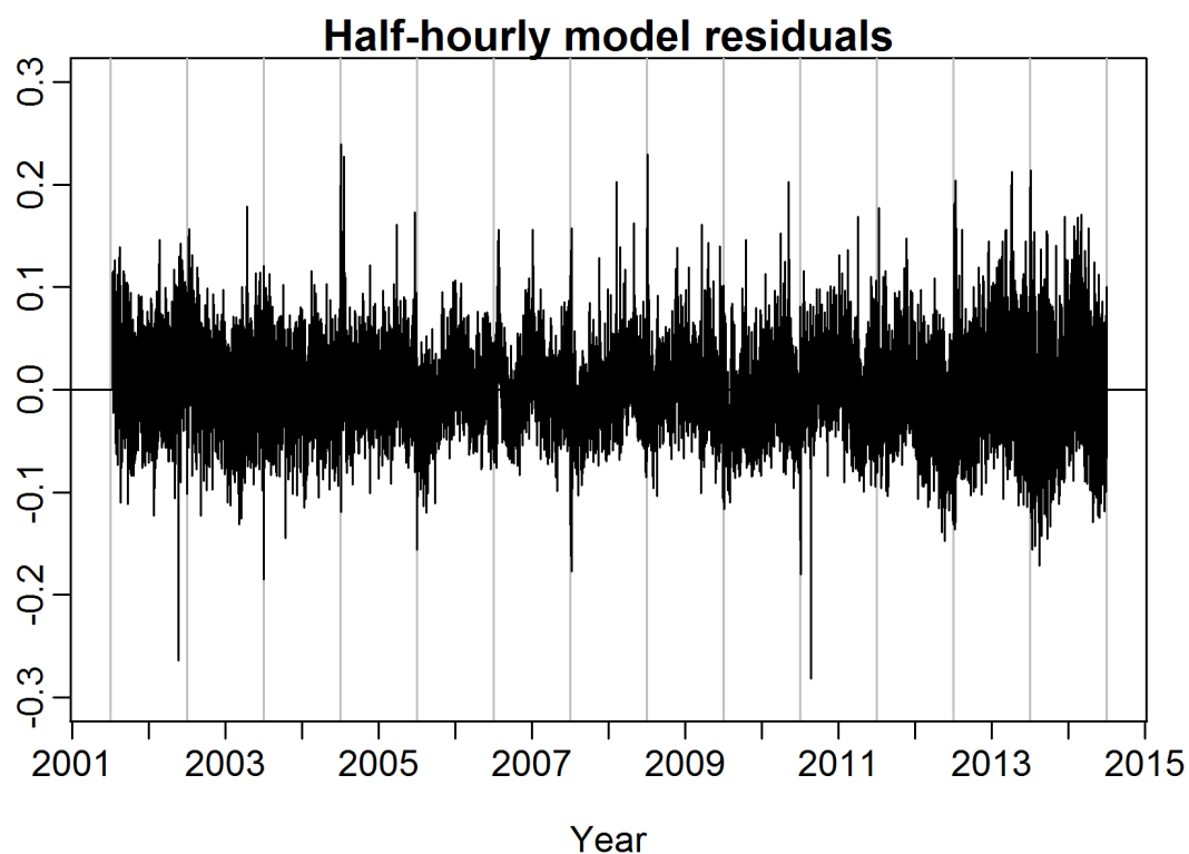
Figure 36: Half-hourly residuals (actual – predicted) from the demand model.
