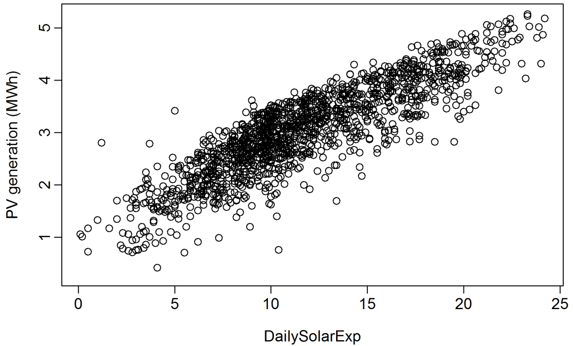
Figure 38: Daily solar PV generation plotted against daily solar exposure data in SA from 2003 to 2011. Only data from April–September are shown.
