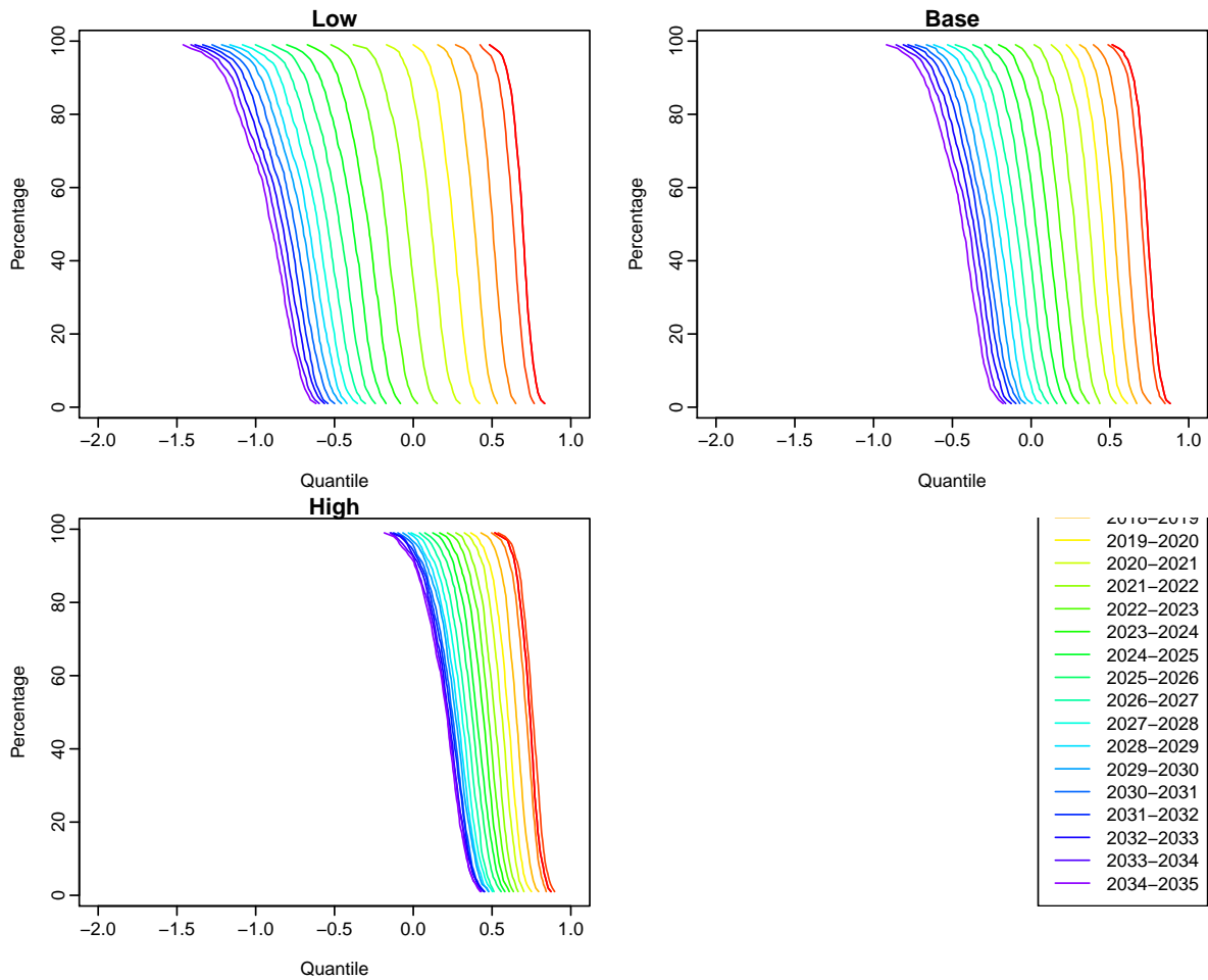
Figure 24: Quantiles of prediction of seasonal minimum demand for 2015/16–2034/35.
