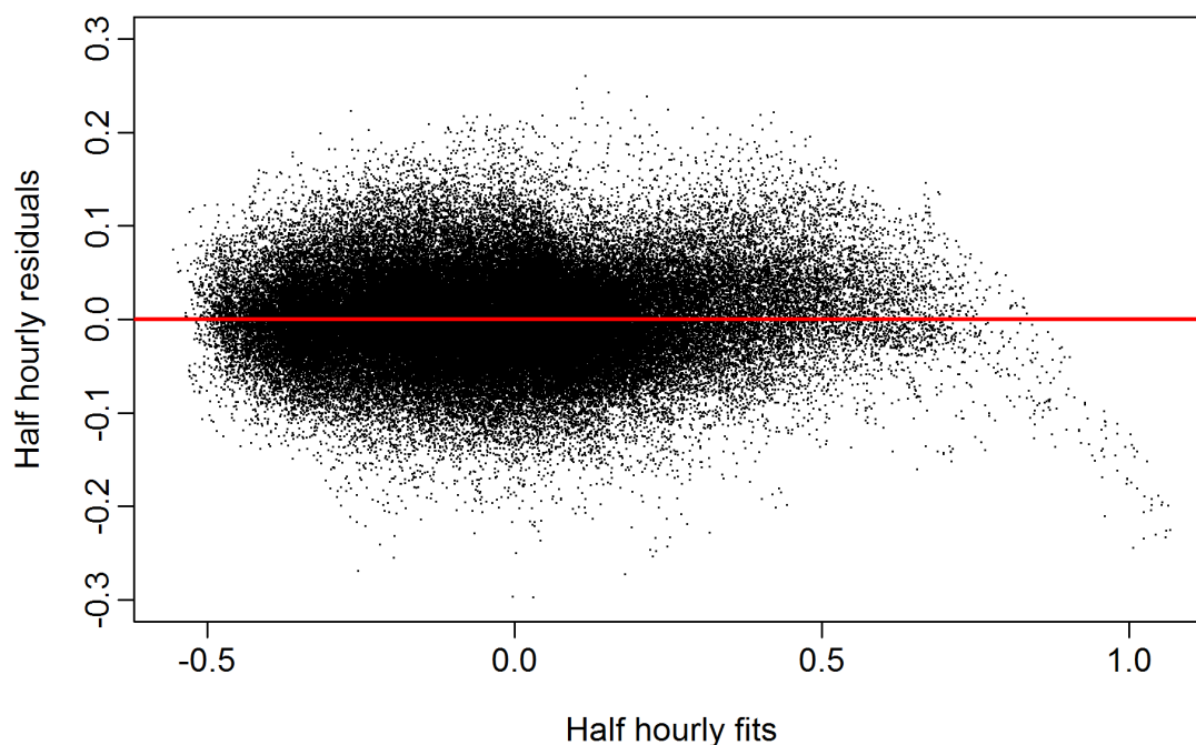
Figure 13: Residuals vs predicted log adjusted demand from the demand model.
