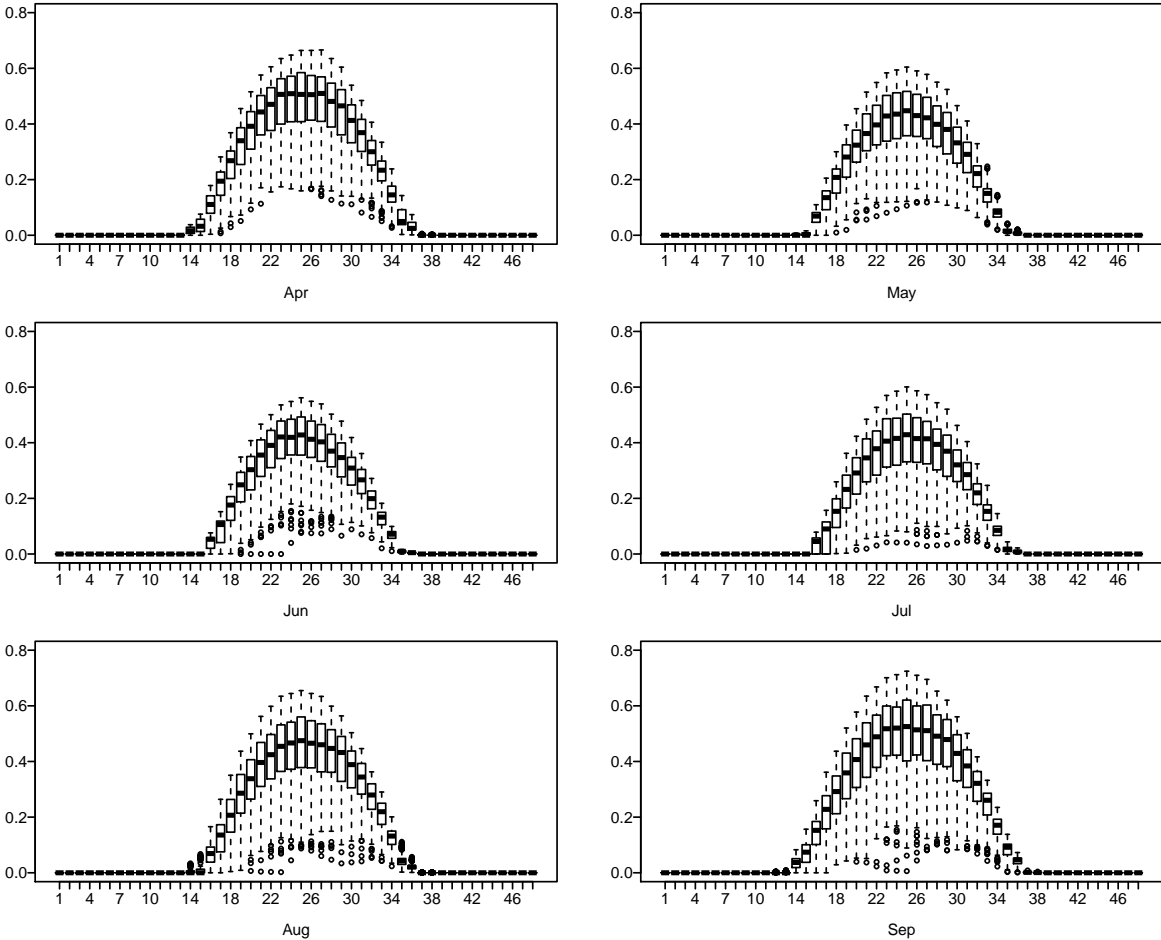
Figure 40: Boxplot of historical PV output based on a 1 MW solar system. Only data from April–September are shown.
