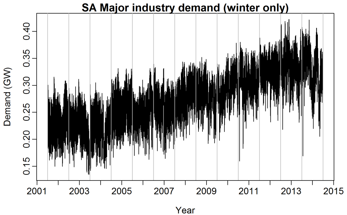
Figure 29: Half-hourly demand data for aggregated major industries from 2002 to 2015.
