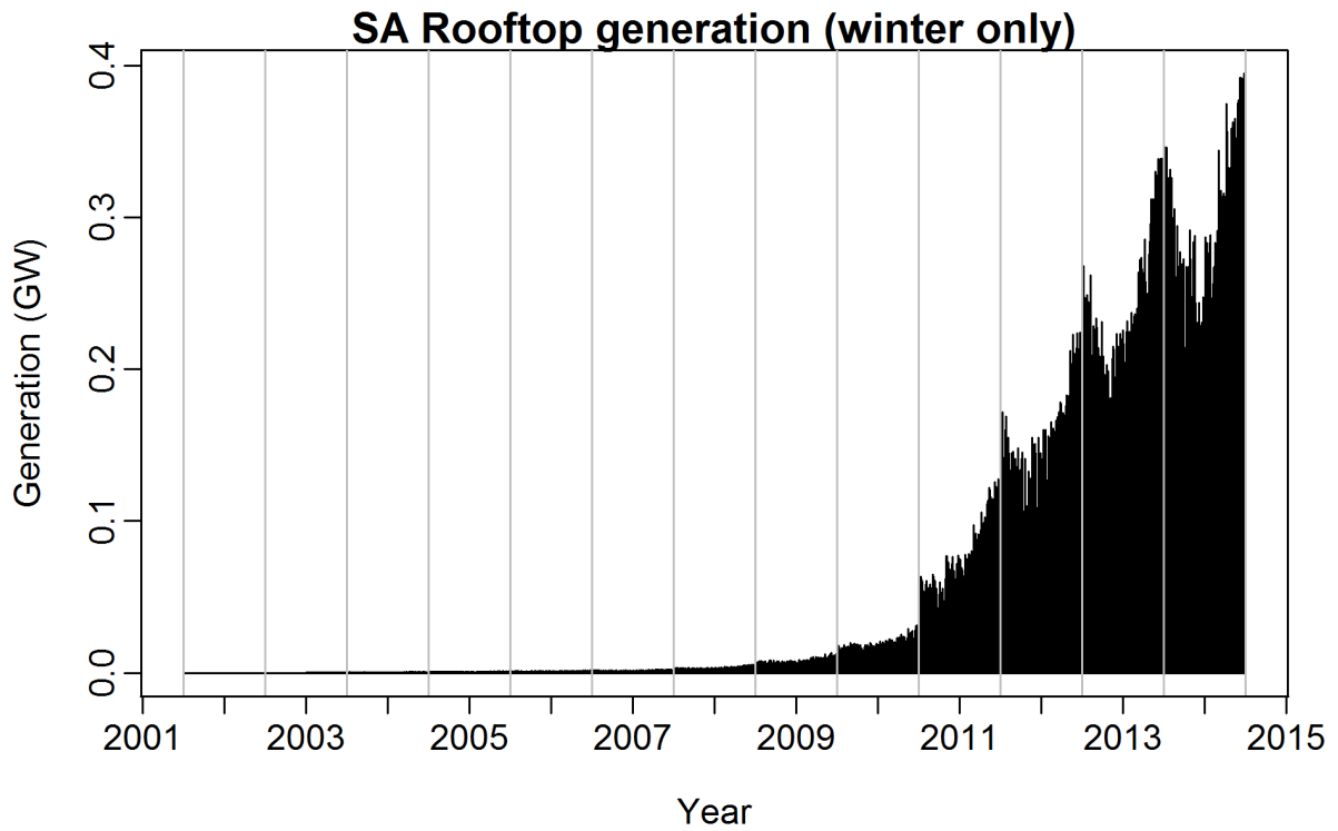
Figure 31: Half-hourly rooftop generation data. 2003–2015.
