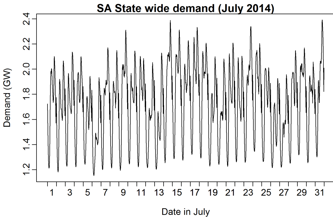
Figure 28: Half-hourly demand data for South Australia, July 2014.
