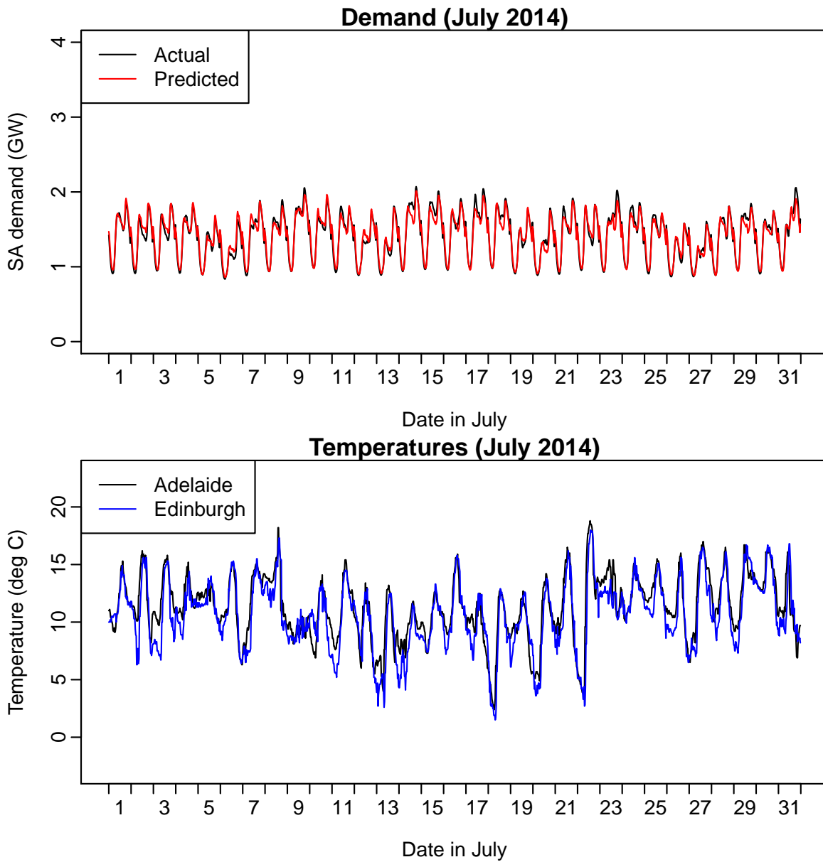
Figure 35: Actual and predicted demand for July 2014.
