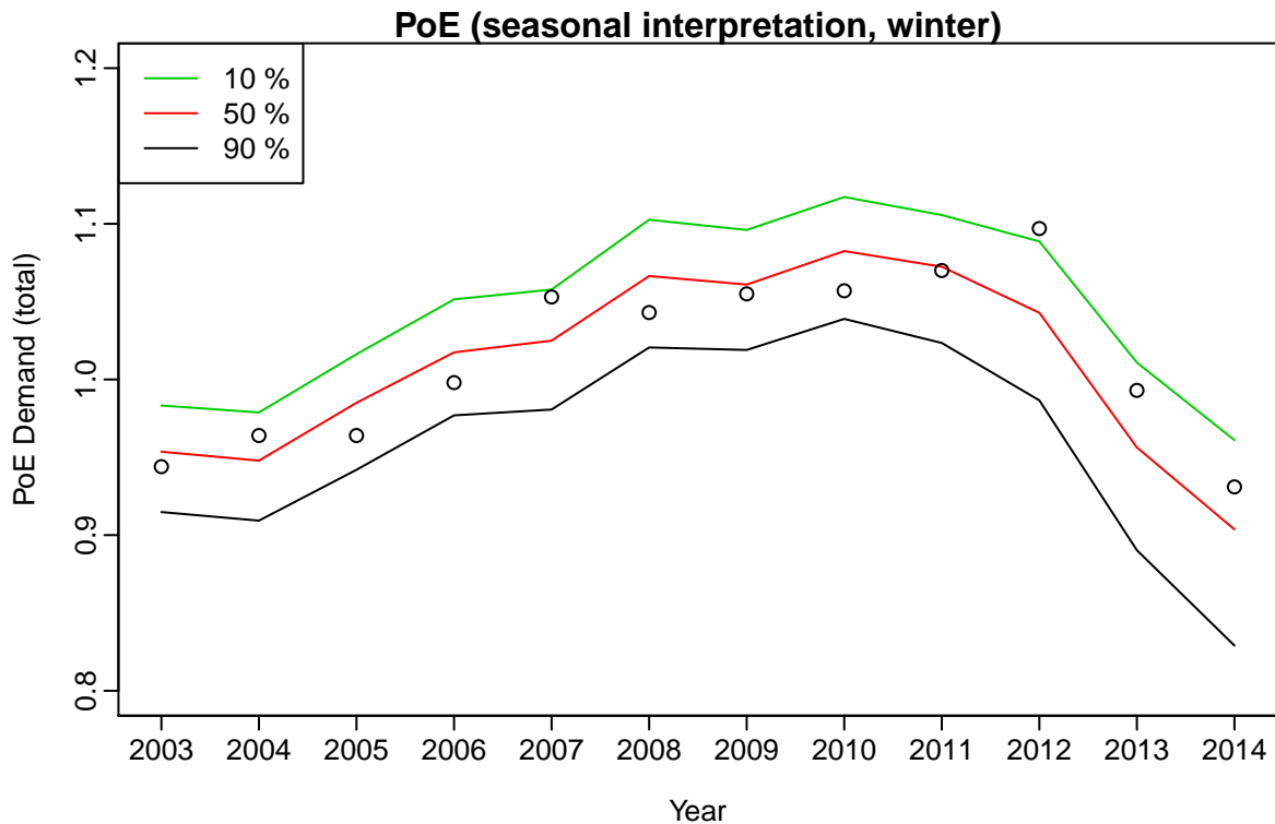
Figure 42: PoE levels of demand excluding offset loads for all years of historical data using known economic values but simulating temperatures.
