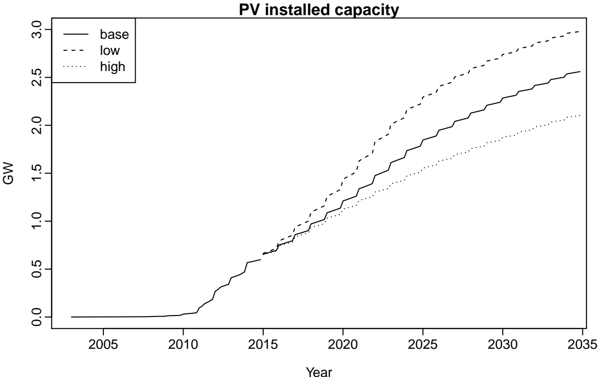
Figure 46: Three scenarios for installed capacity of rooftop photo-voltaic (PV) cells.
